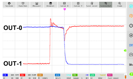
Switching time: H to L / R_L = 22Ω
