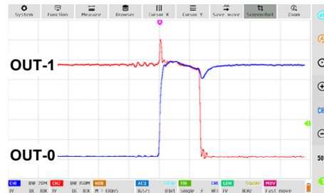
Switching time: L to H / R_L = 22Ω
