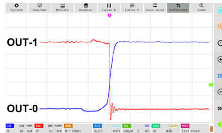
Switching time: L to H / R_L = Open
