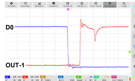
PD: H to L / R_L = 22Ω
