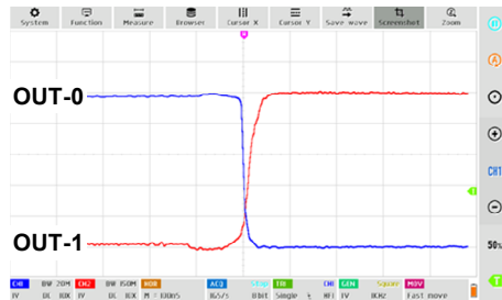
Switching time: H to L / R_L = Open
