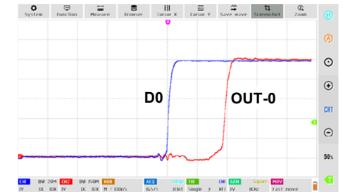
PD: L to H / R_L = Open
