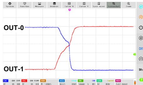
Switching time: H to L / R_L = 1K
