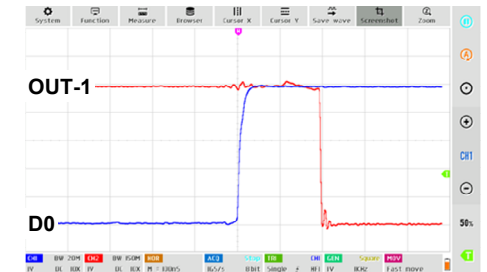
PD: L to H / R_L = Open
