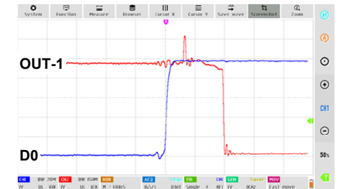
PD: L to H / R_L = 22Ω
