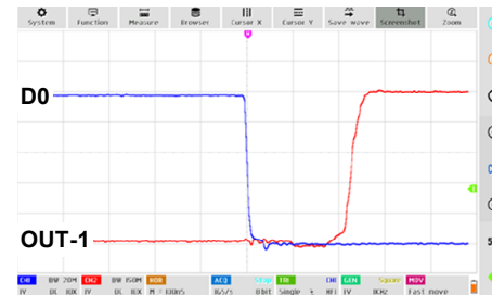
PD: H to L / R_L = Open
