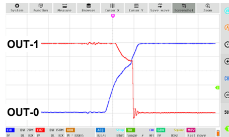
Switching time: L to H / R_L = 1K
