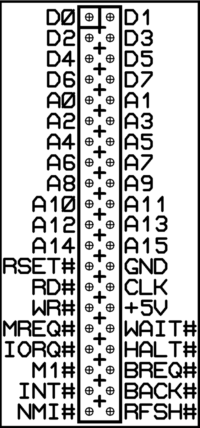
TOP Silk
